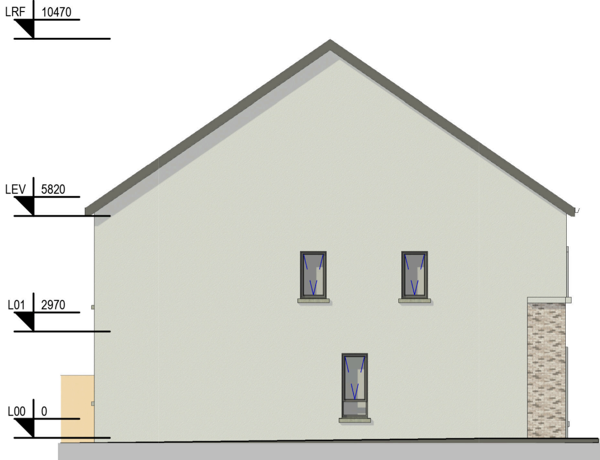
4: BHA1 Left Side Elevation Scale - 1 : 100
