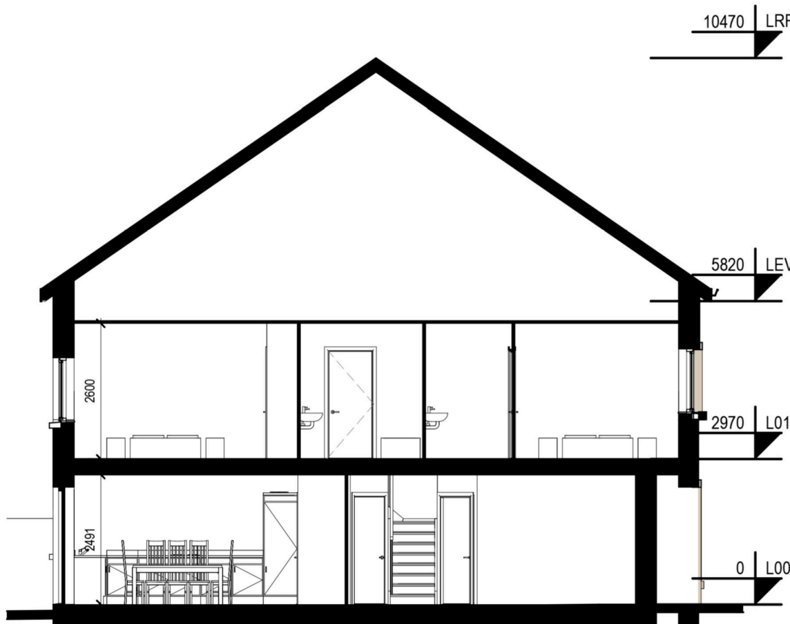
8: BHA1 Section Scale - 1 : 100
