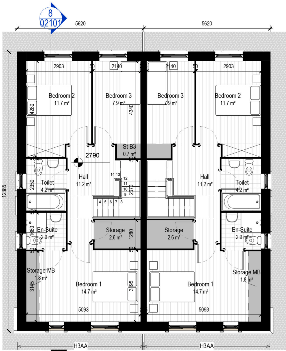
2: BHA1 - L01 First Floor Plan Scale - 1 : 100
