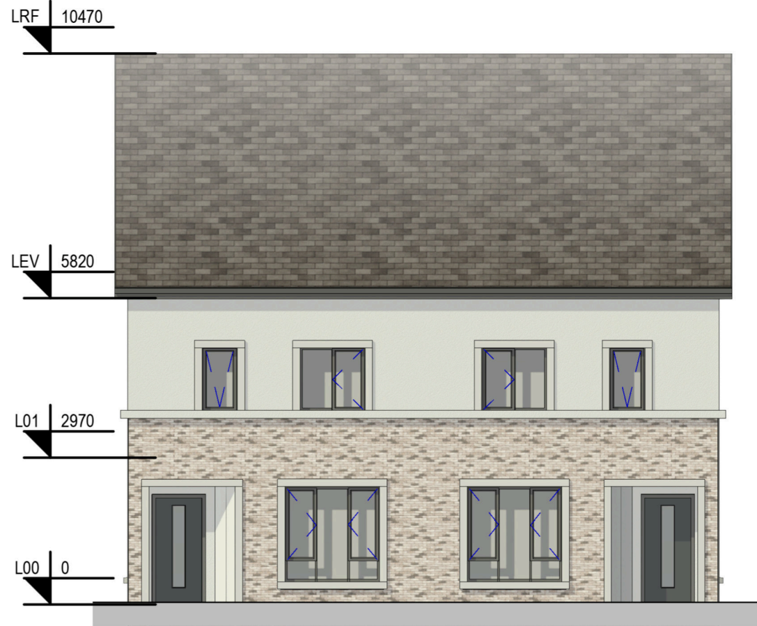
3: BHA1 Front Elevation Scale - 1 : 100
