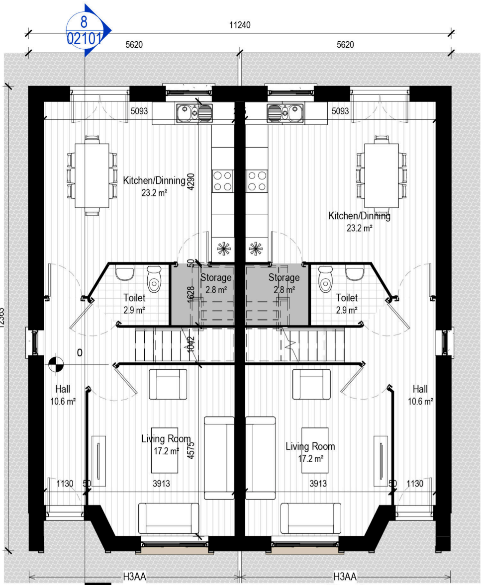
1: BHA1 - L00 Ground Floor Plan Scale - 1 : 100
