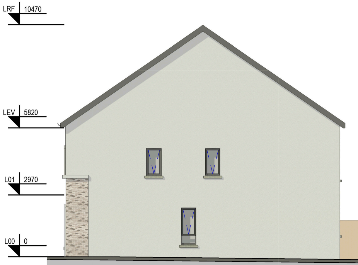
6: BHA1 Right Side Elevation Scale - 1 : 100
