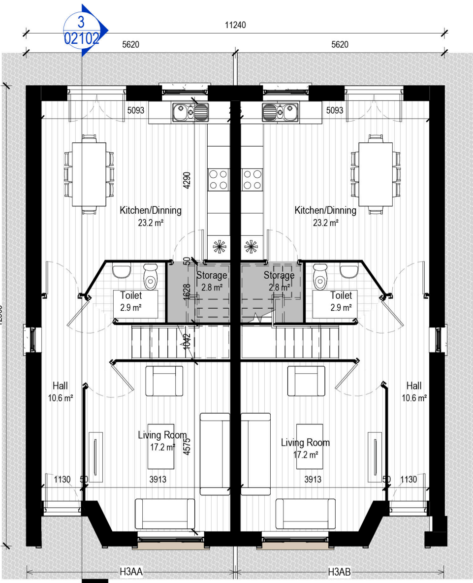
1: BHA2 - L00 Ground Floor Plan Scale - 1 : 100
