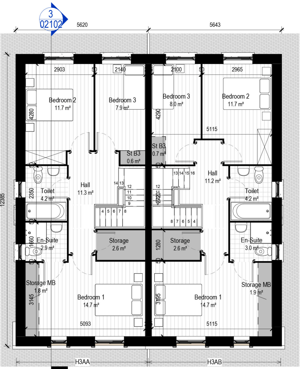
2: BHA2 - L01 First Floor Plan Scale - 1 : 100
