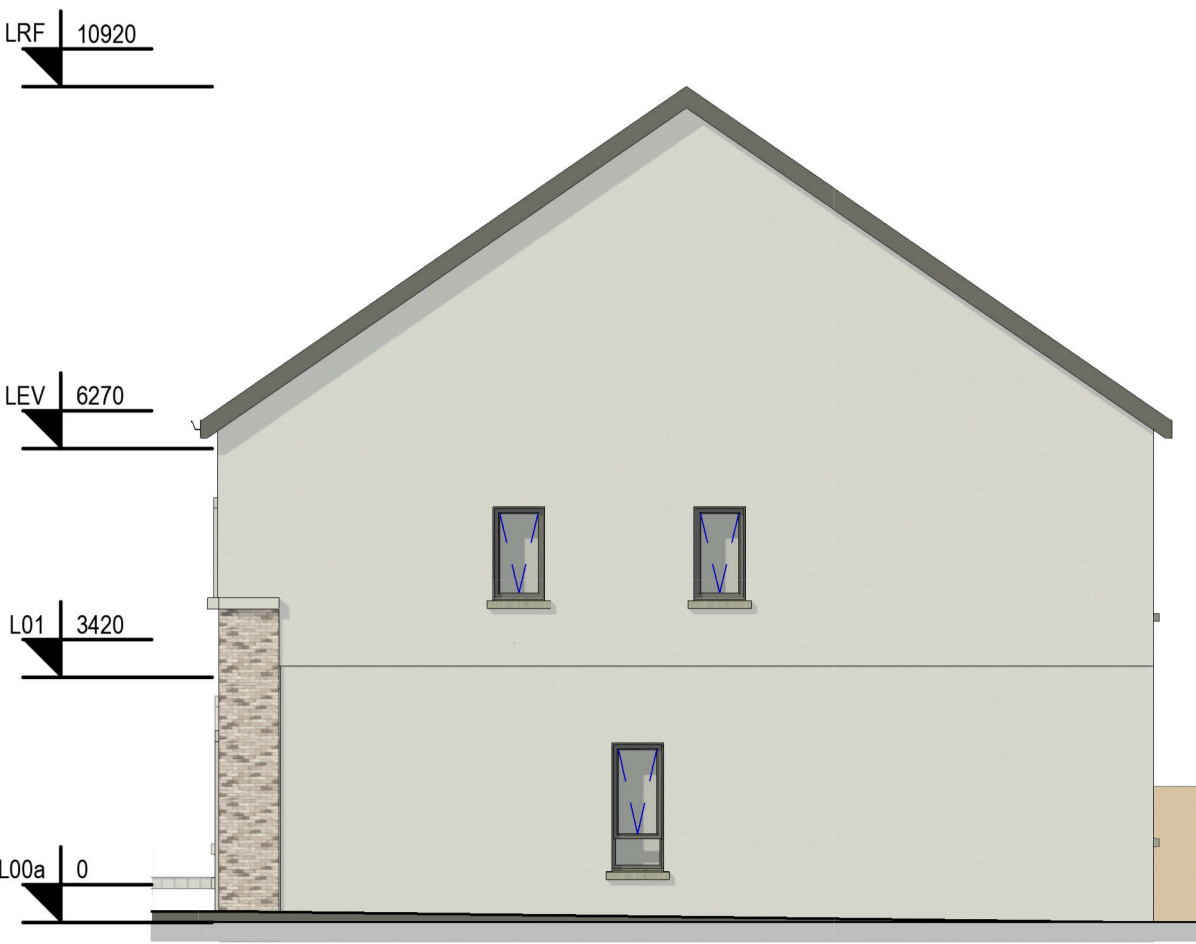
7: BHA2 Right Side Elevation Scale - 1 : 100
