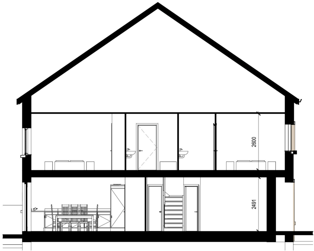
3: BHA2 Section Scale - 1 : 100
