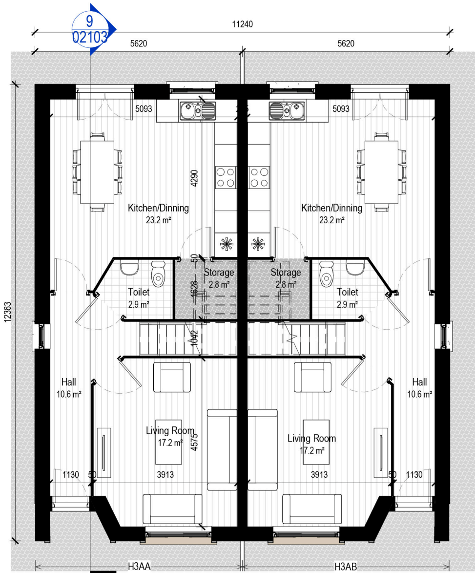
1: BHA3 - L00 Ground Floor Plan Scale - 1 : 100
