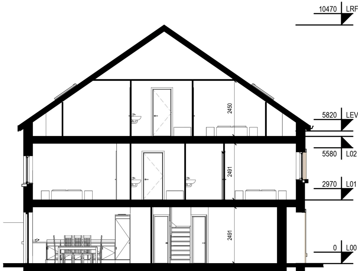
9: BHA3 Section Scale - 1 : 100
