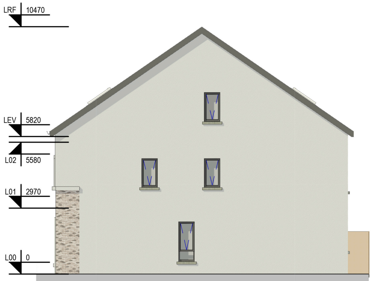
8: BHA3 Right Side Elevation Scale - 1 : 100
