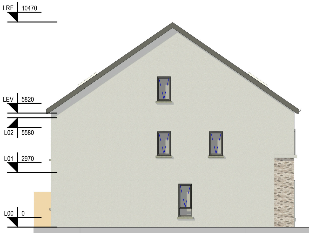
6: BHA3 Left Side Elevation Scale - 1 : 100
