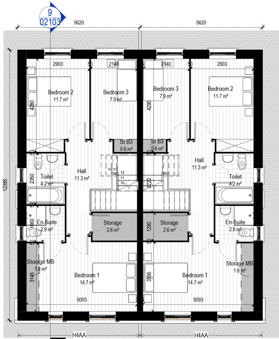
2: BHA3 - L01 First Floor Plan Scale - 1 : 100
