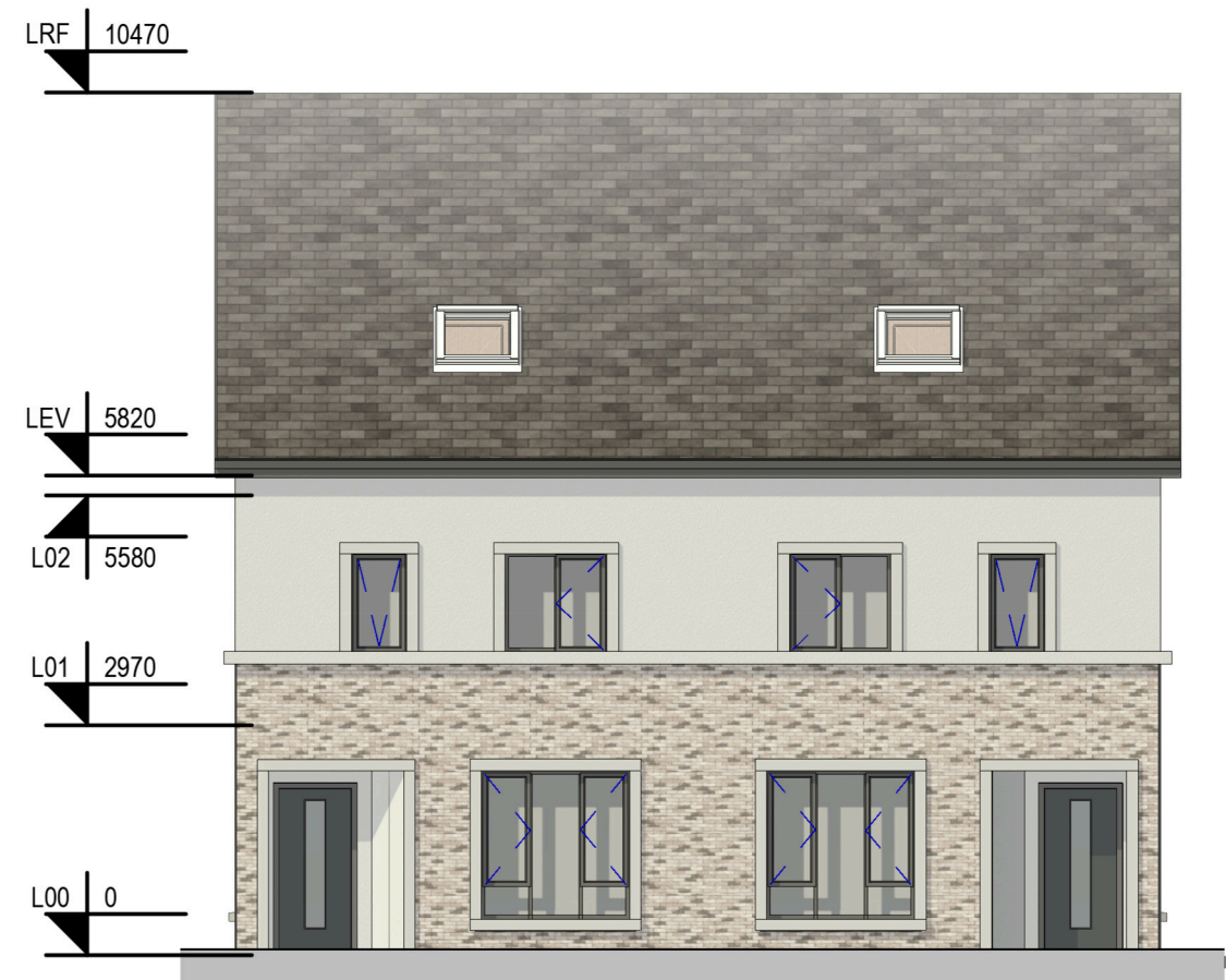
5: BHA3 Front Elevation Scale - 1 : 100
