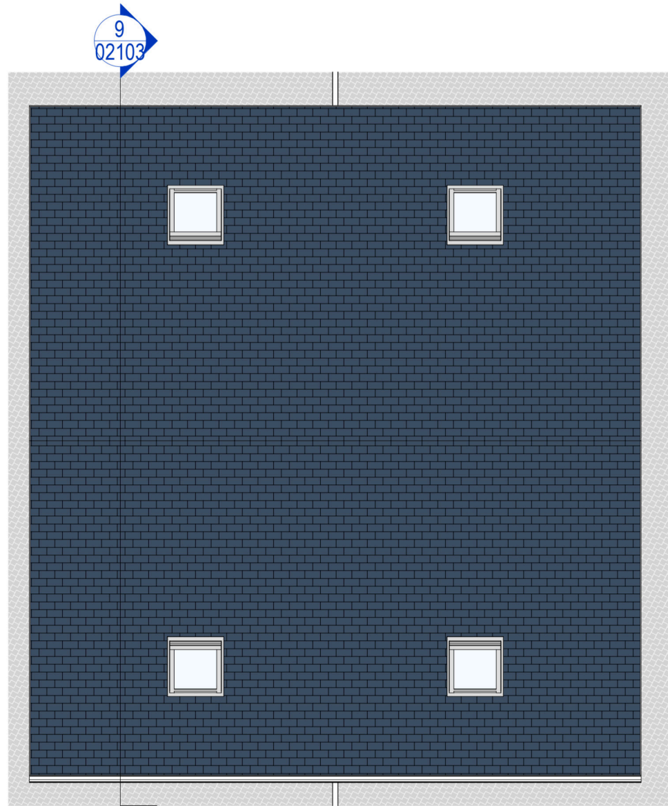
3: BHA3 - LRF Roof Plan Scale - 1 : 100
