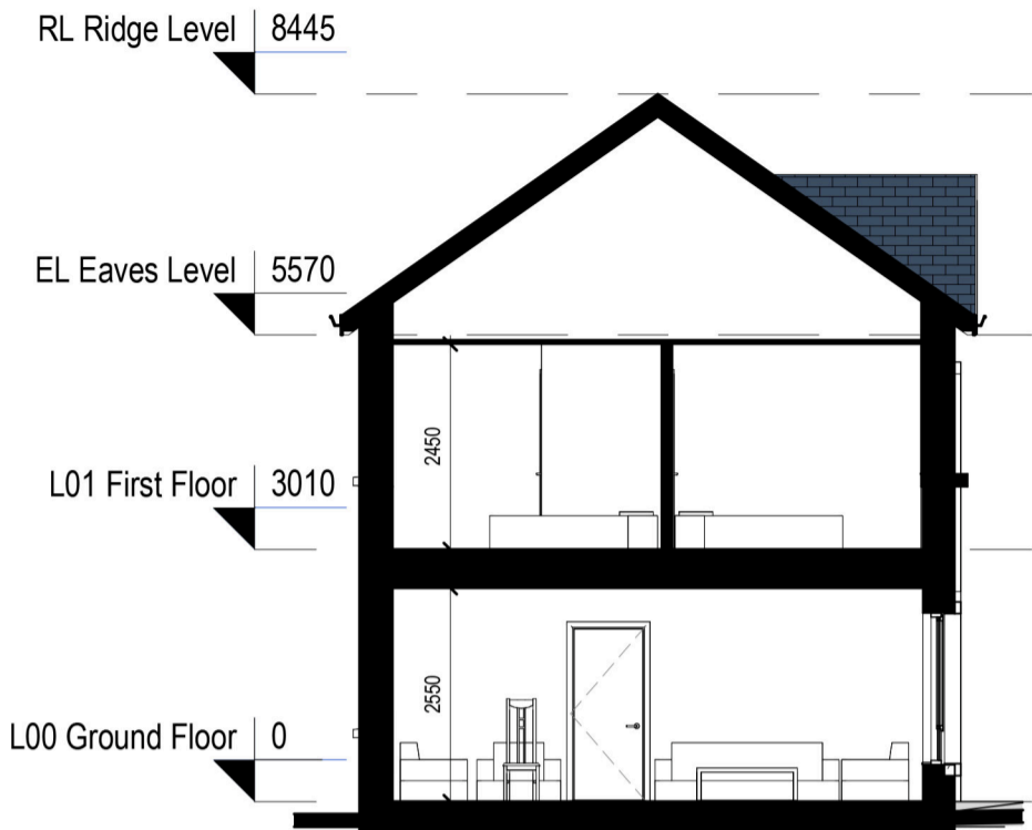
4: BHB1 Section Scale - 1 : 100
