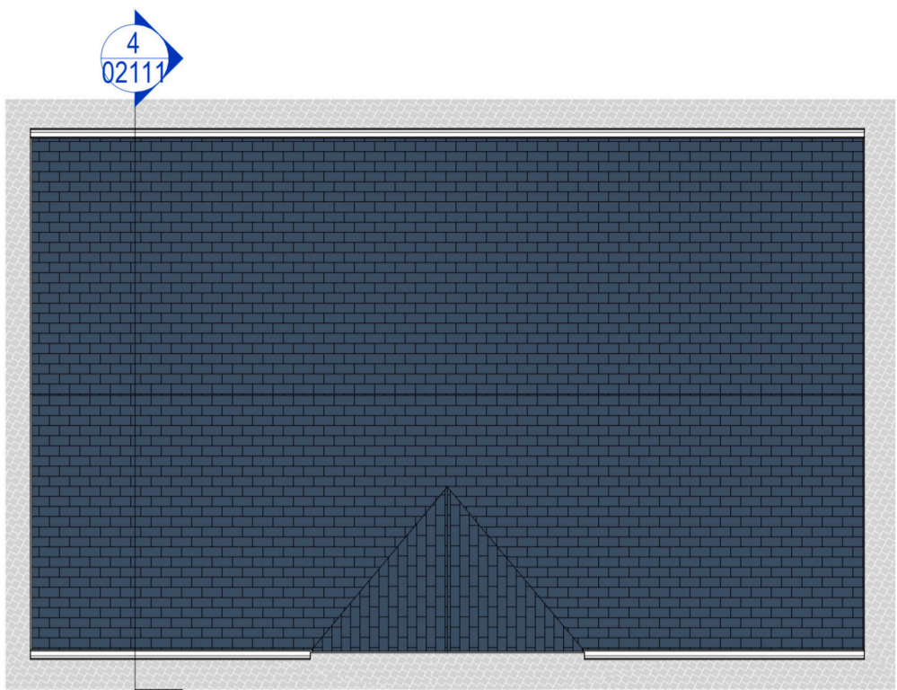
3: BHB1 - LRF Roof Plan Scale - 1 : 100
