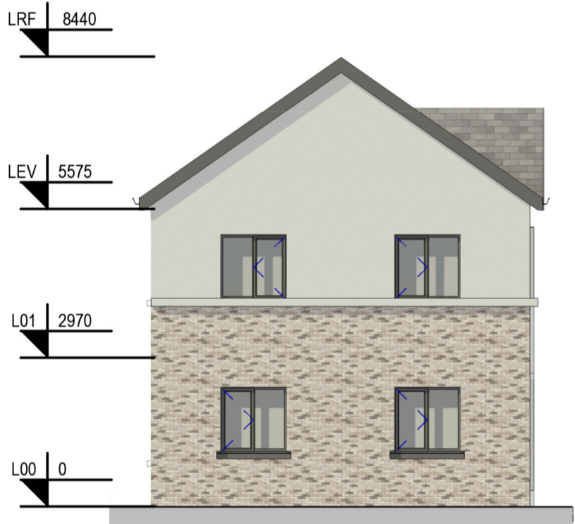
6: BHB1 Left Side Elevation Scale - 1 : 100
