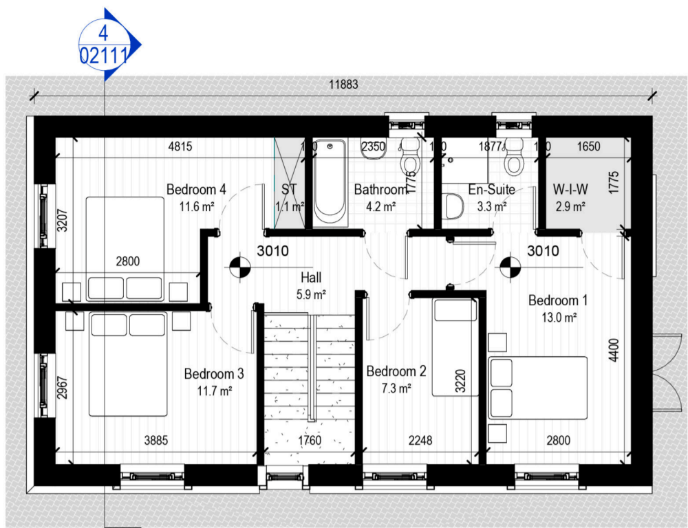
2: BHB1 - L01 First Floor Plan Scale - 1 : 100
