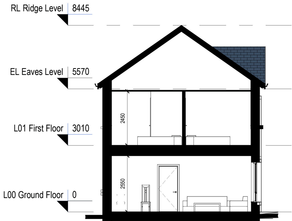
4: BHB2 Section Scale - 1 : 100
