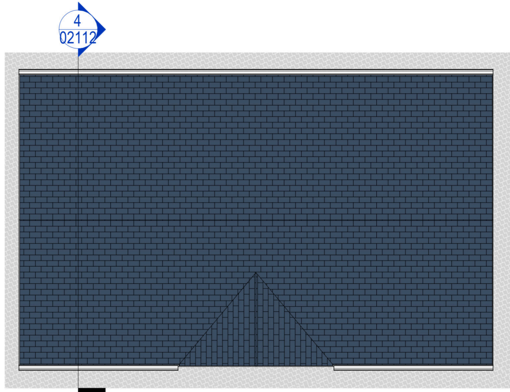
3: BHB2 - LRF Roof Plan Scale - 1 : 100
