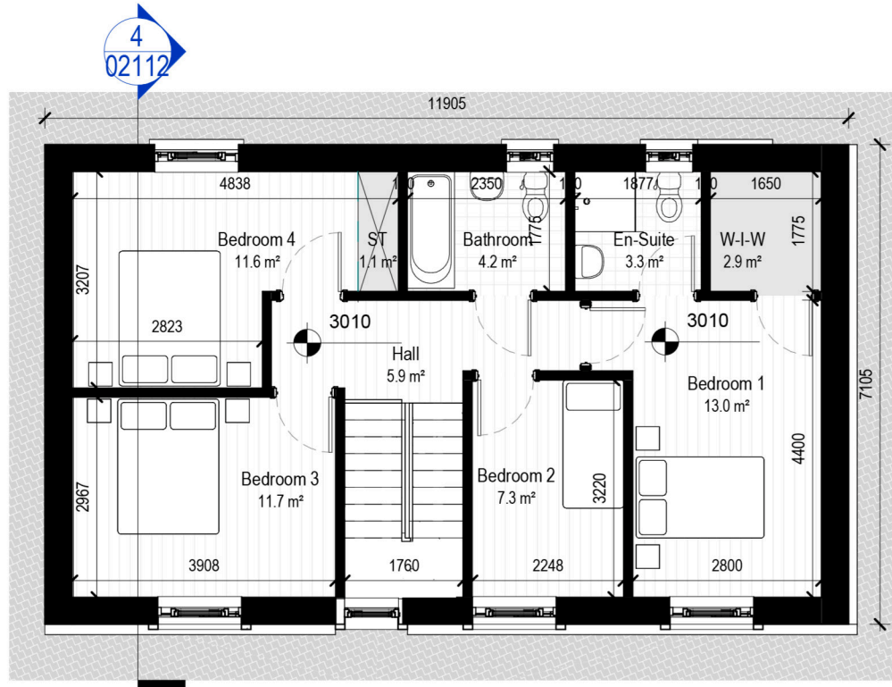
2: BHB2 - L01 First Floor Plan Scale - 1 : 100
