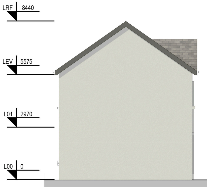
6: BHB2 Left Side Elevation Scale - 1 : 100
