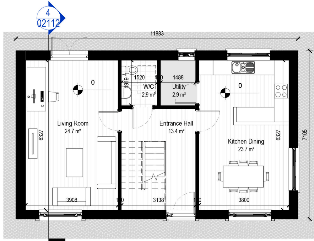
1: BHB2 - L00 Ground Floor Plan Scale - 1 : 100
