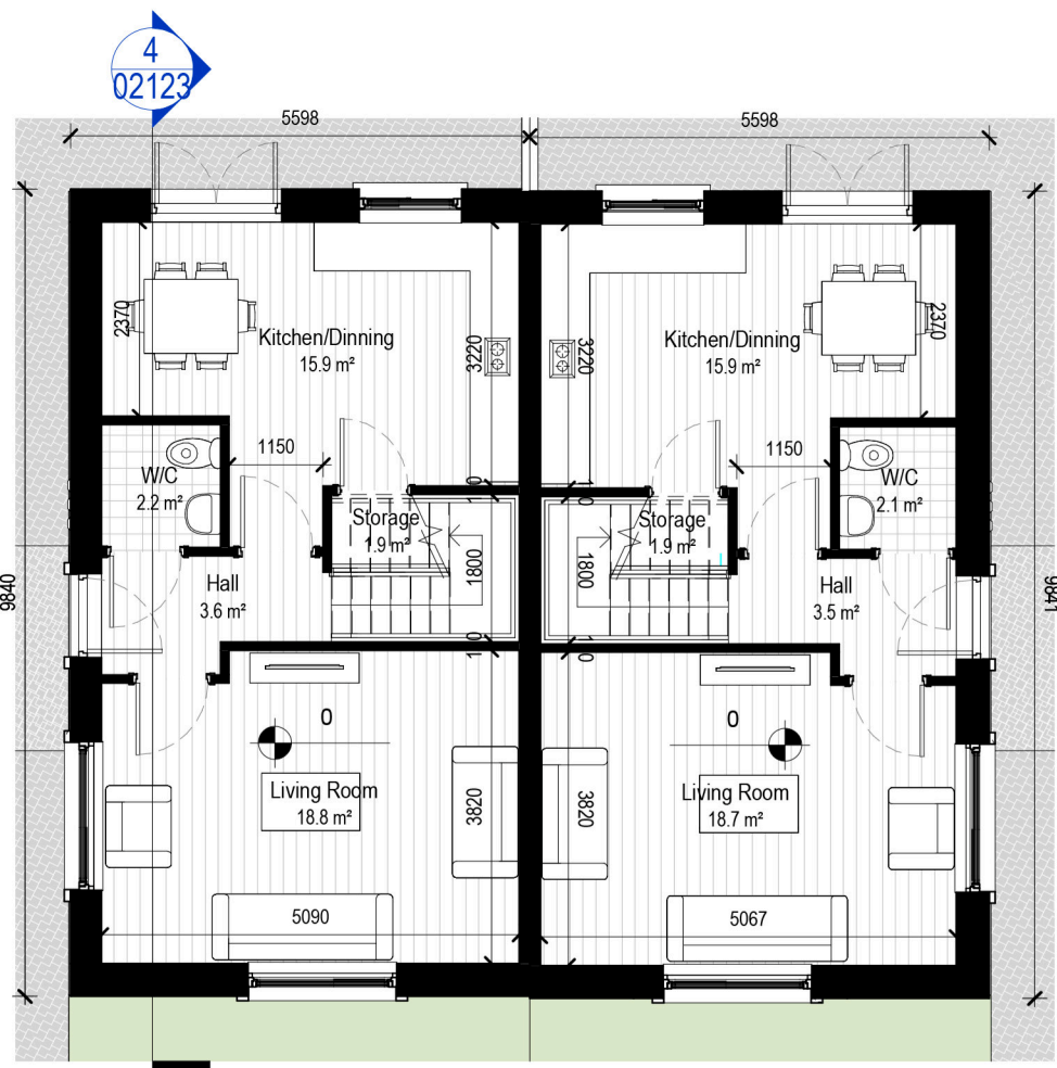
1: BHC3 - L00 Ground Floor Plan Scale - 1 : 100
