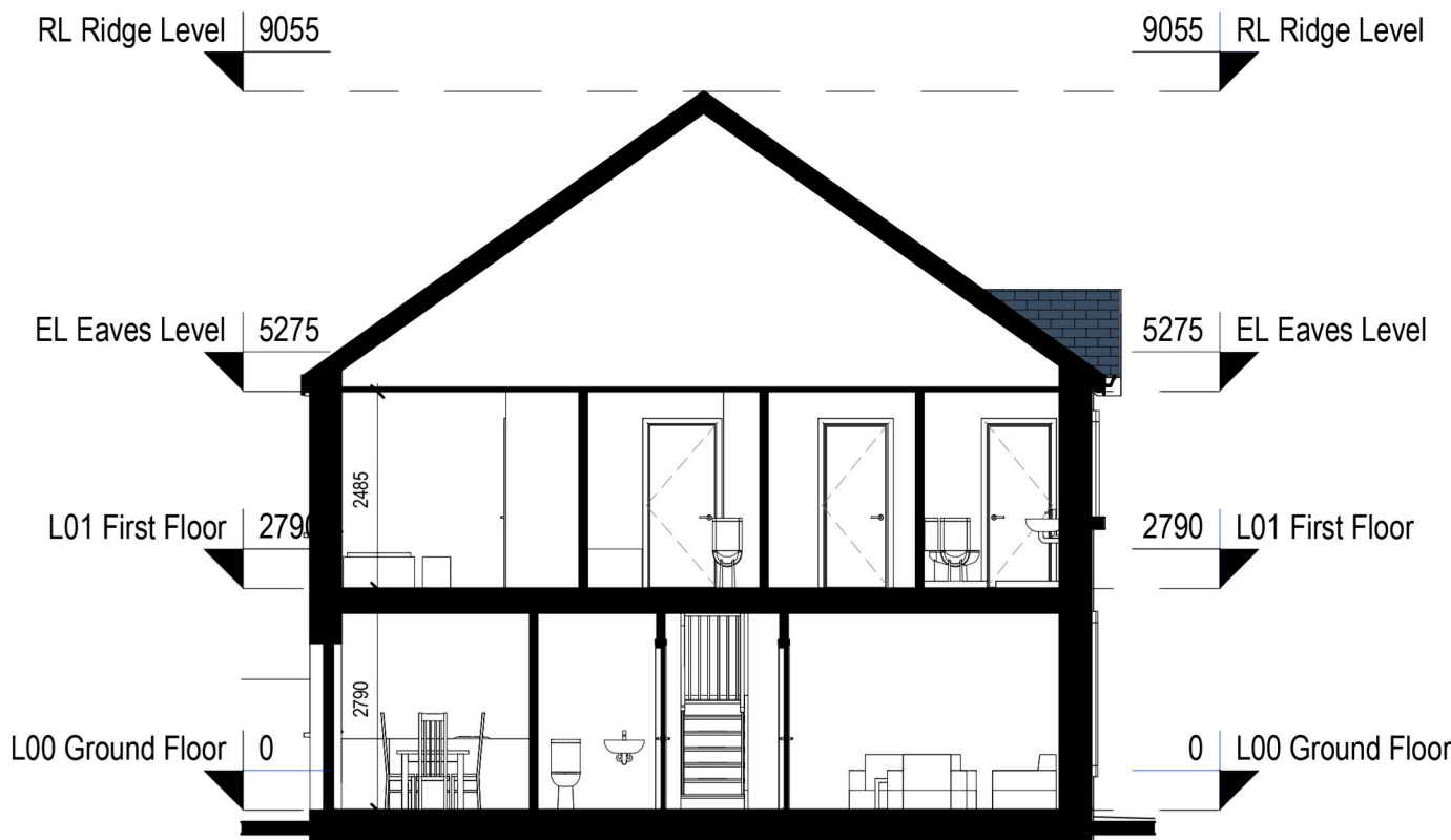
4: BHC3 Section Scale - 1 : 100
