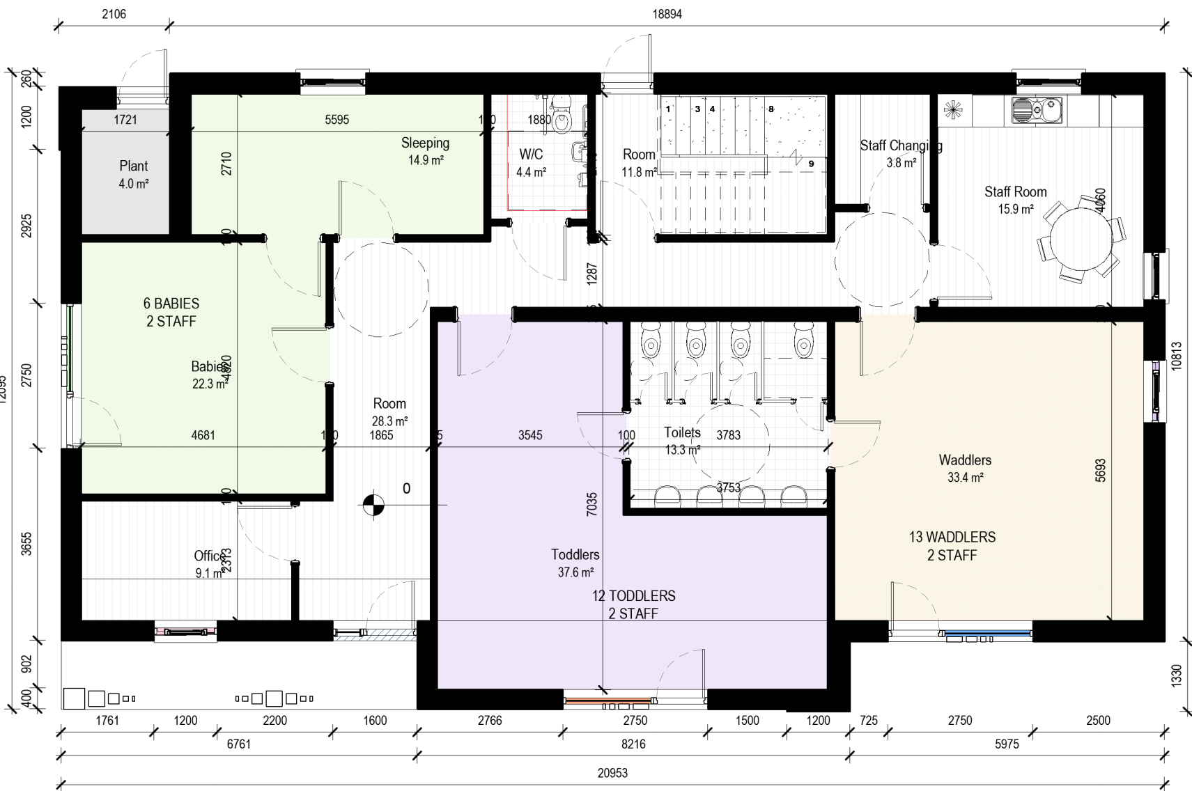
1: BX01 Creche - L00 Ground Floor Plan Scale - 1 : 100
