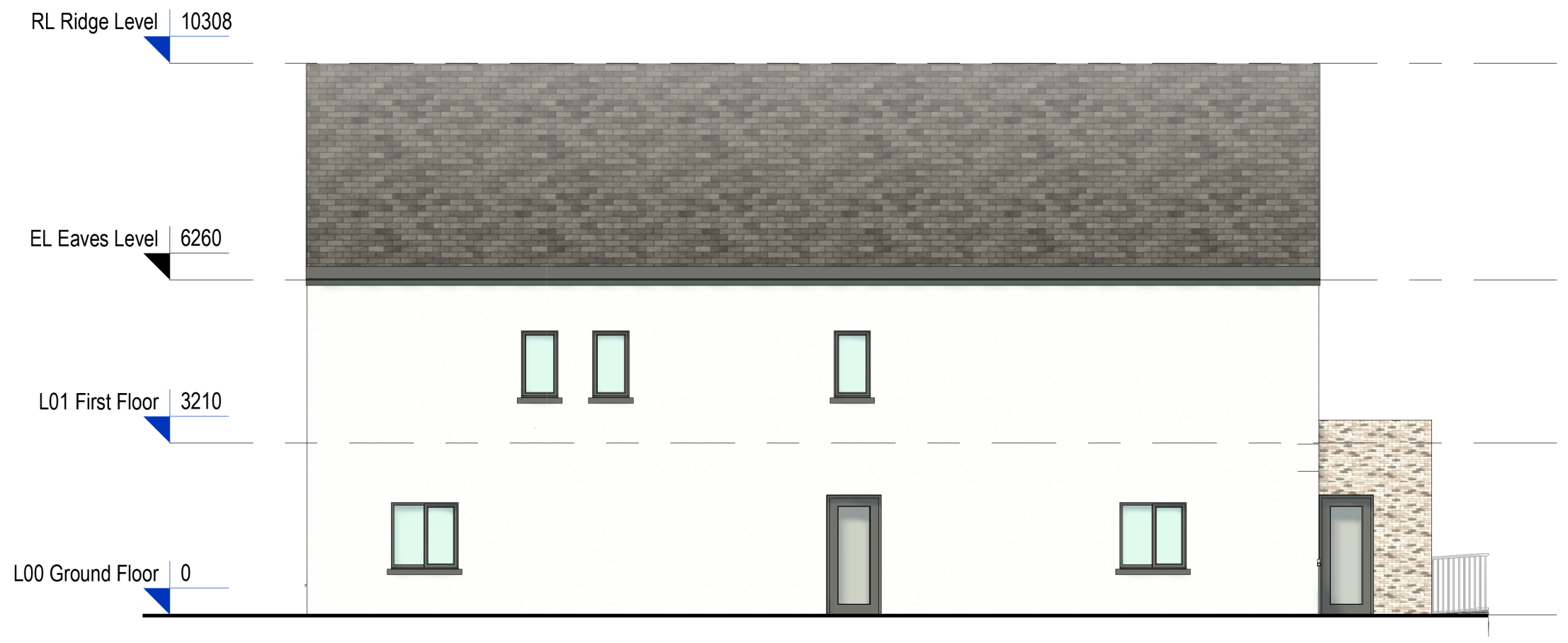
6: BX01 Rear/ West Elevation Scale - 1 : 100
