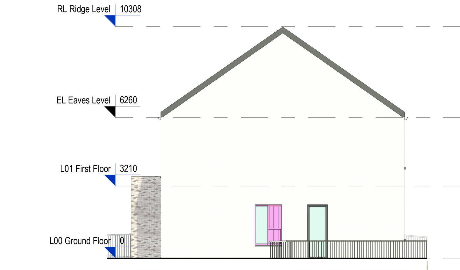
7: BX01 North Elevation Scale - 1 : 100
