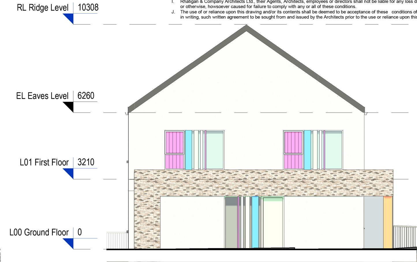
5: BX01 Street / South Elevation Scale - 1 : 100
