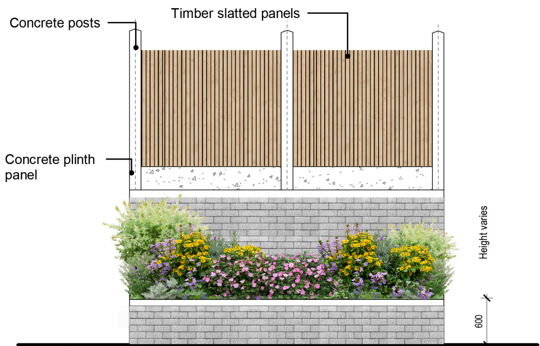
4: Retaining Wall Detail Scale - 1 : 50
